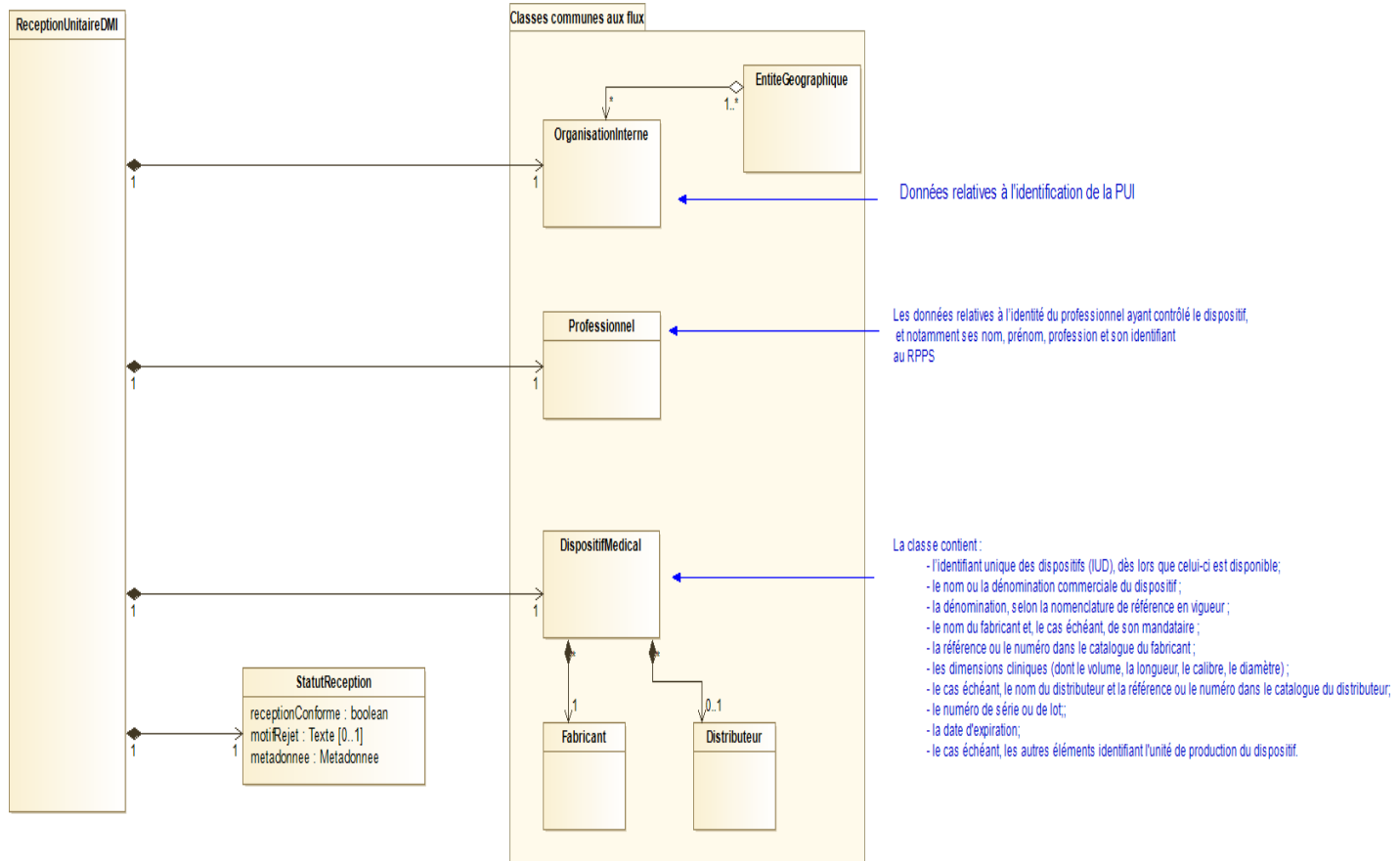
Figure 31 Flux 5b - ReceptionUnitaireDMI
