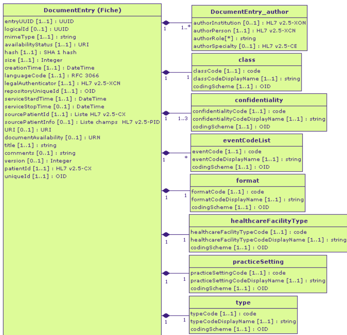
Figure 8: Classe XDS DocumentEntry
