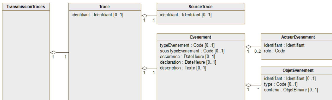
Figure 8 Flux 1 - TransmissionTrace
